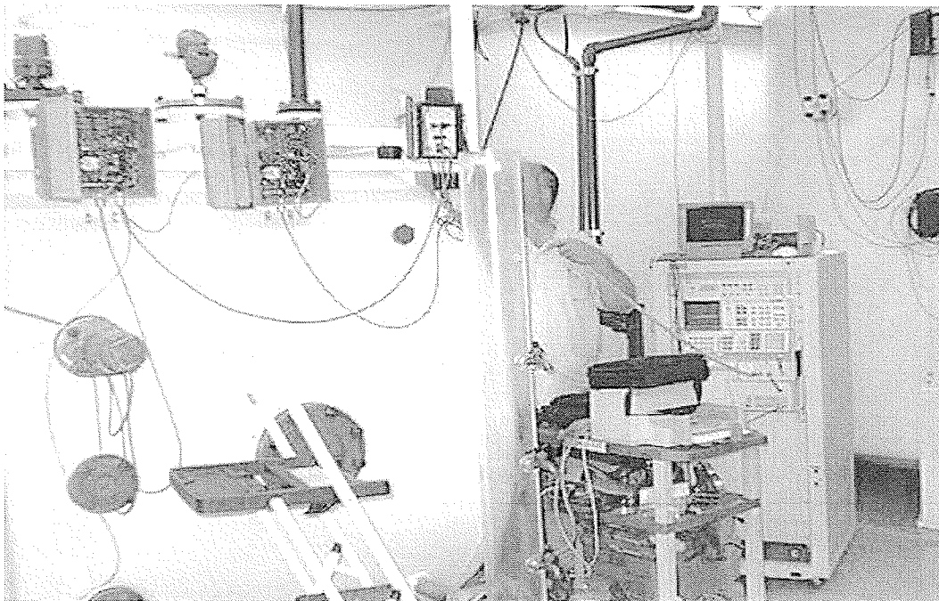
FIGURE 2c - TEST SETUP IN A METAL TANK AT MAGNETROL FACILITY IN DOWNERS GROVE, ILLINOIS
