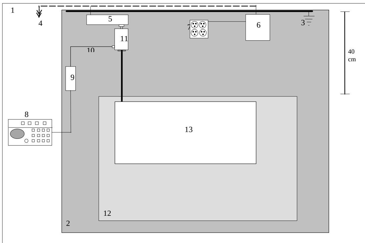
Figure 2. Conducted Emissions Test Setup Diagram
