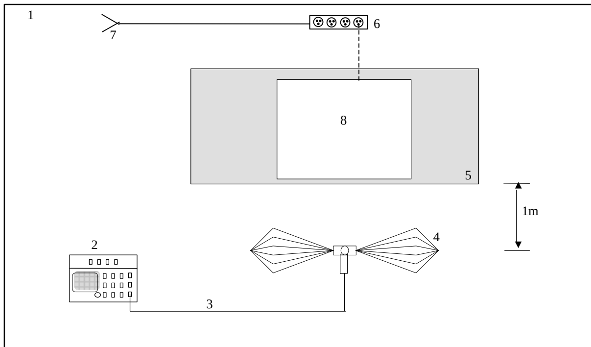
Figure 3. Radiated Emissions Frequency ID Test Setup Diagram
