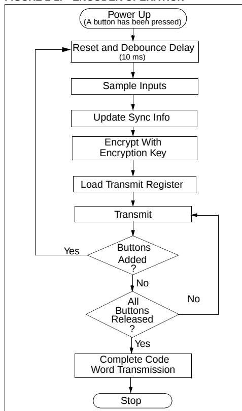
FIGURE 2-2: ENCODER OPERATION
