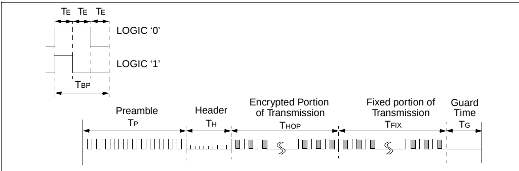
FIGURE 8-3: PREAMBLE/HEADER FORMAT
