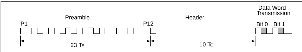
FIGURE 8-3: PREAMBLE/HEADER FORMAT
