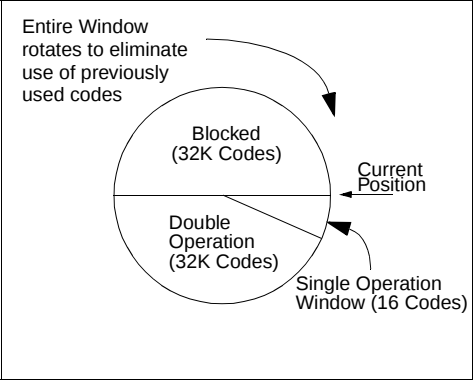
FIGURE 7-3: SYNCHRONIZATION WINDOW
