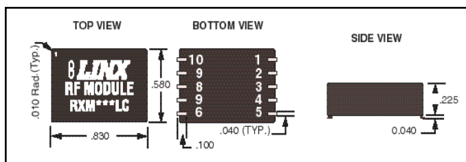
figure 2: LC Series Receiver Package Dimensions
