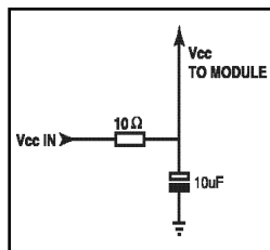
figure 15: Supply Filter
