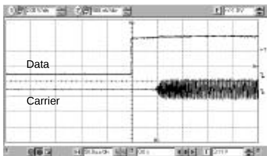
figure 3: Typical RF power into 50Ω
