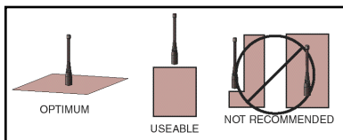
figure 16: Groundplane orientation
