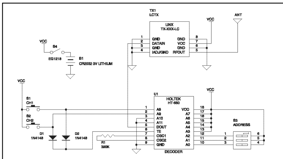
figure 12: Basic Remote Control Transmitter Circuit
