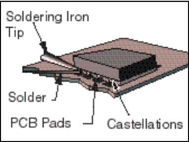
Figure 7: LC-TX Soldering Technique
