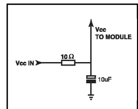
figure 10: Supply Filter
