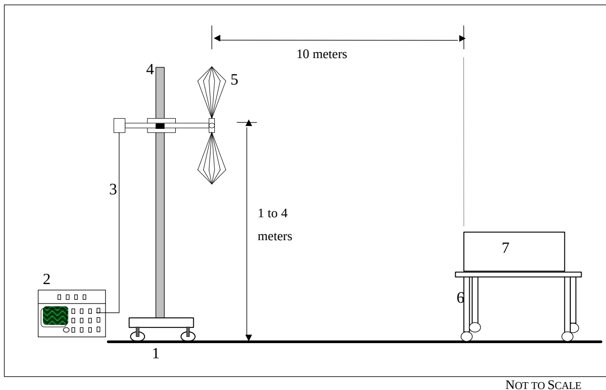
Figure 3. Radiated Emissions (OATS) Test Setup Diagram
