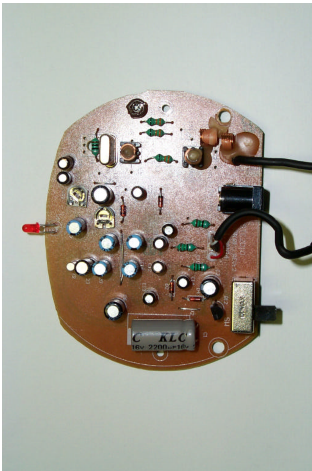
Figure 7.6 PCB Component Side
