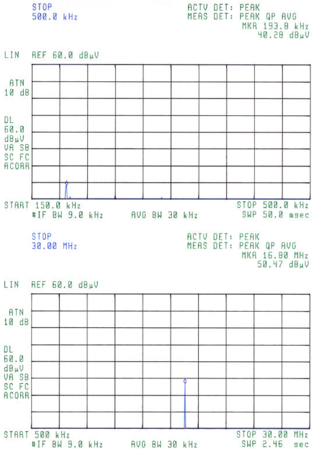
Figure 5.1 Line Conducted
