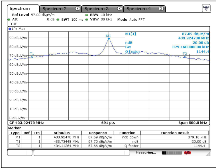
20dB bandwidth
