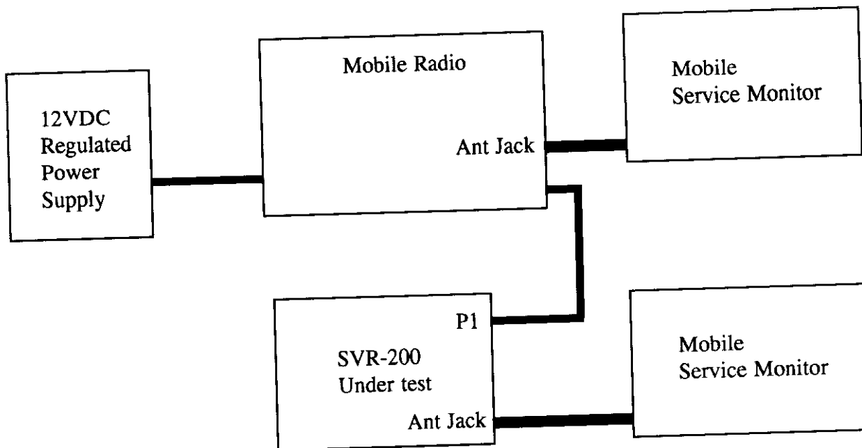
Figure 1 Test Equipment Set up
