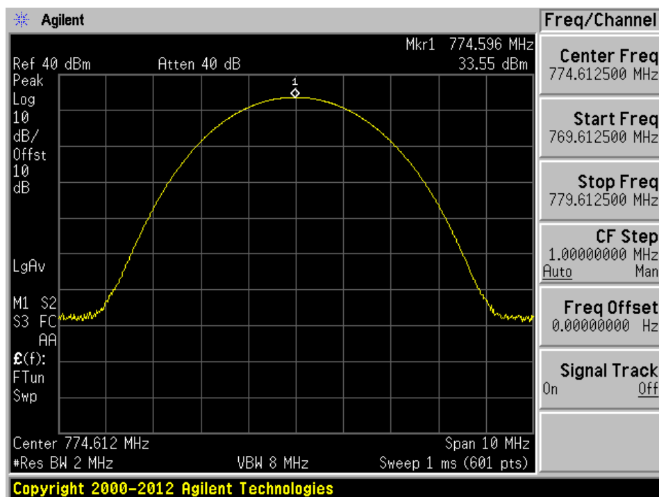
Channel 3 - 774.6125 MHz
