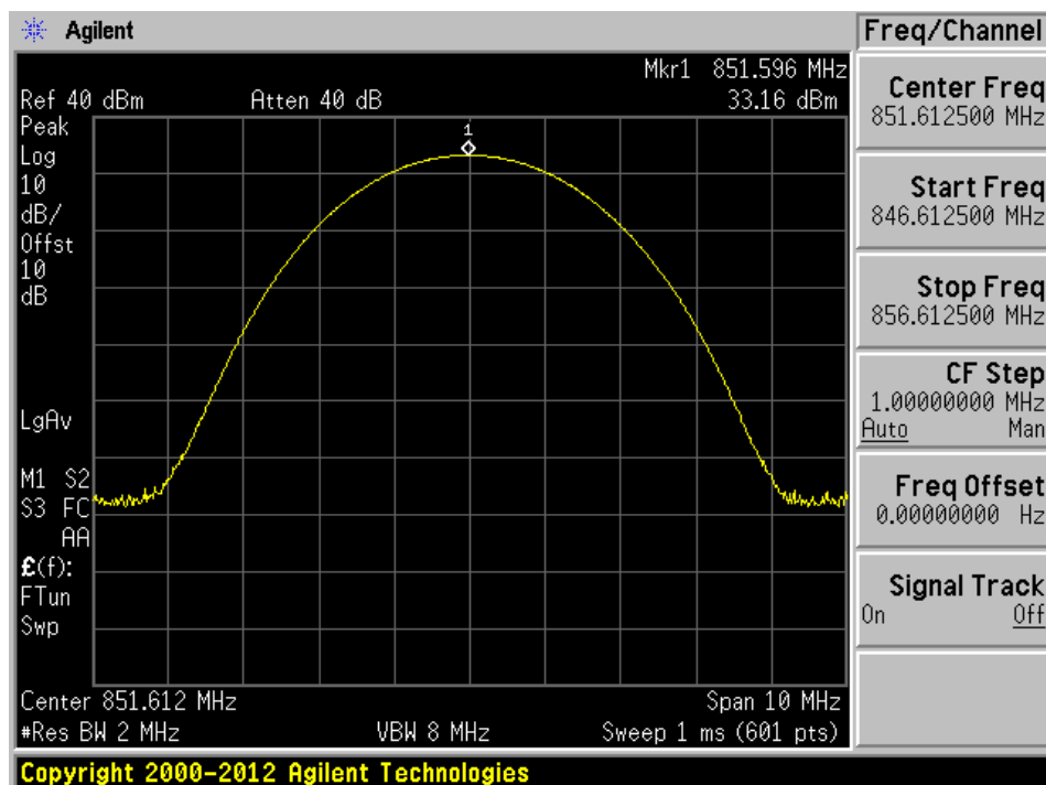
Channel 4 - 851.6125 MHz
