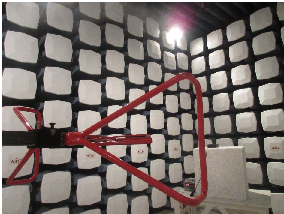
Radiated Emission below 1 GHz (SVR-300M) – Rear View
