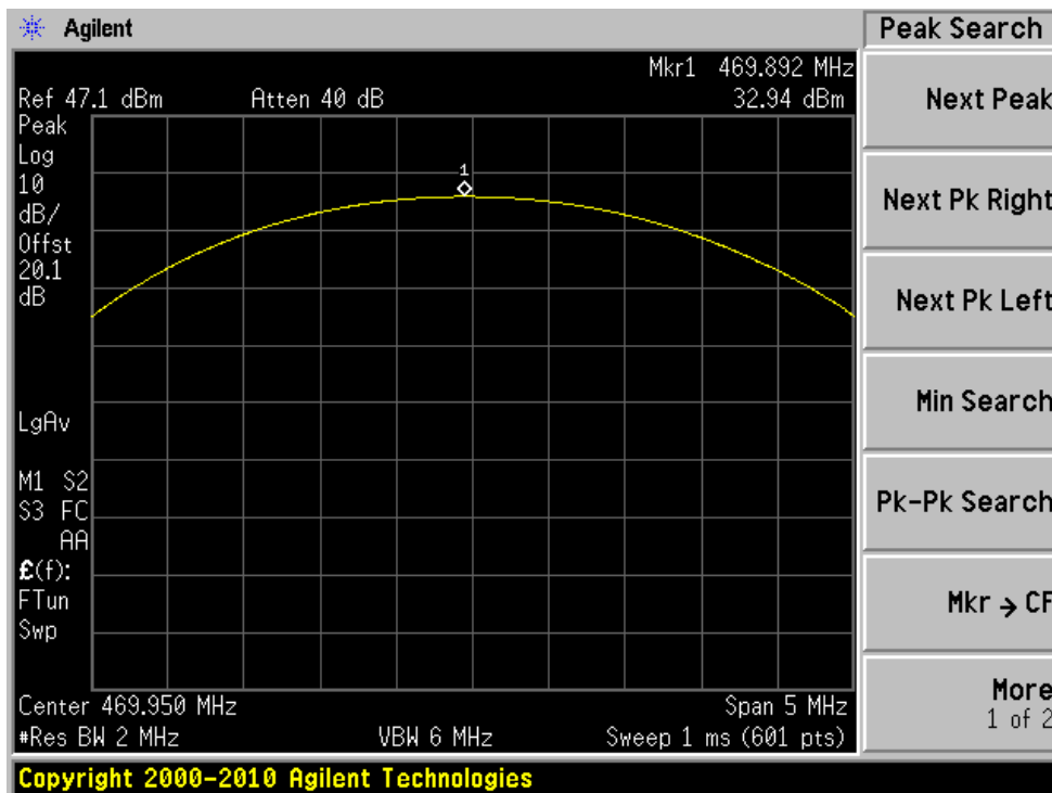
Channel 4: 469.95 MHz
