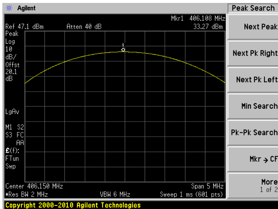
Channel 1: 406.15MHz
