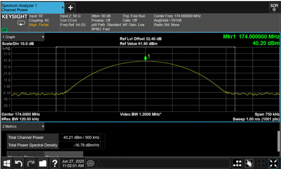
Figure 5 174 MHz:
