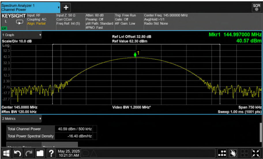
Figure 3 145 MHz:
