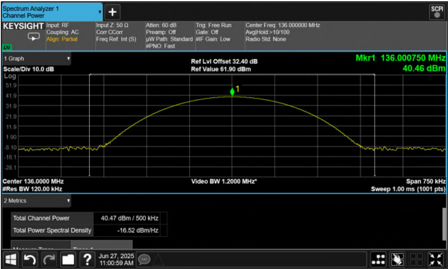
Figure 2 - 136 MHz:
