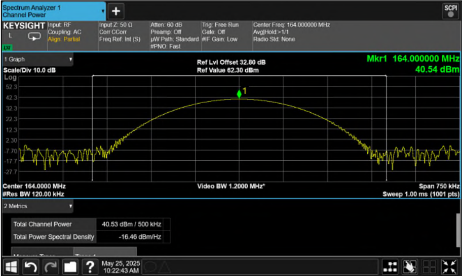
Figure 4 - 164 MHz:
