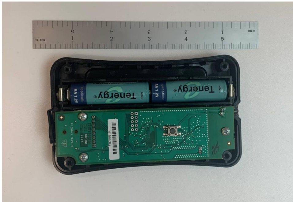
Assembly
