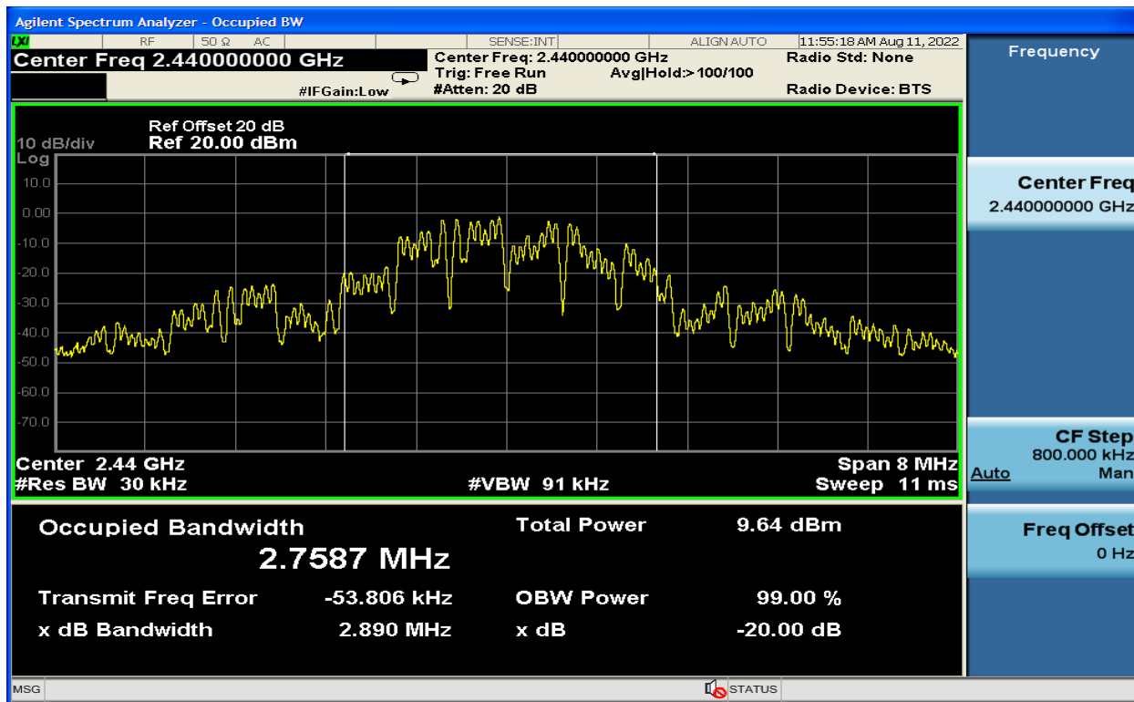
Plot 6-2: 99% Bandwidth, 2440 MHz
