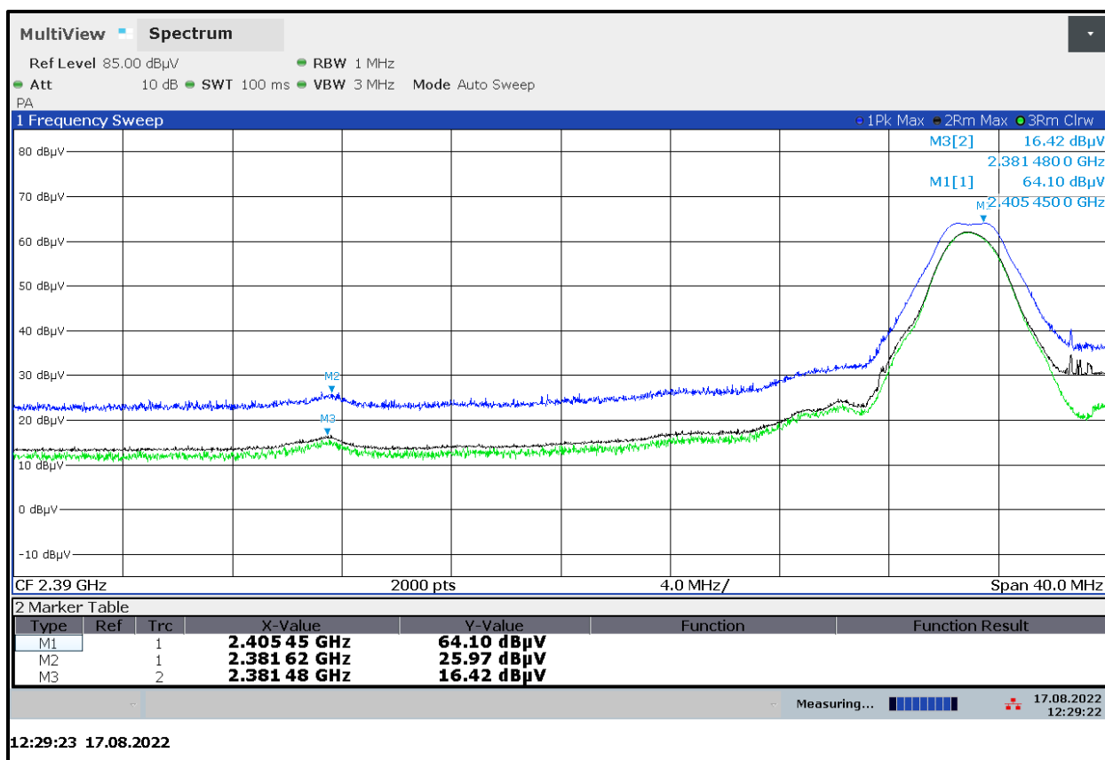
Plot 4-1: Lower Band Edge
