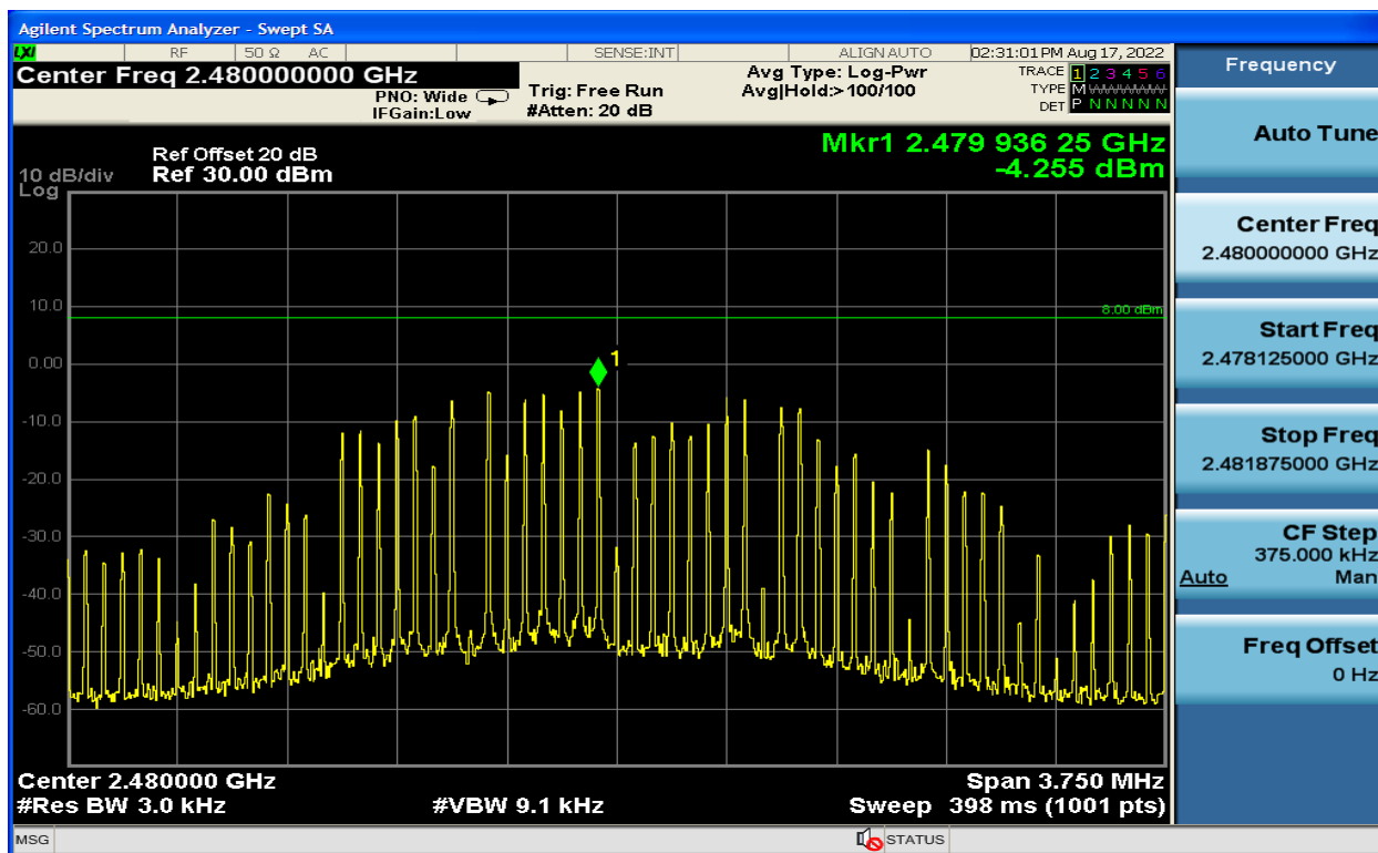
Plot 8-3: Power Spectral Density – 2480 MHz
