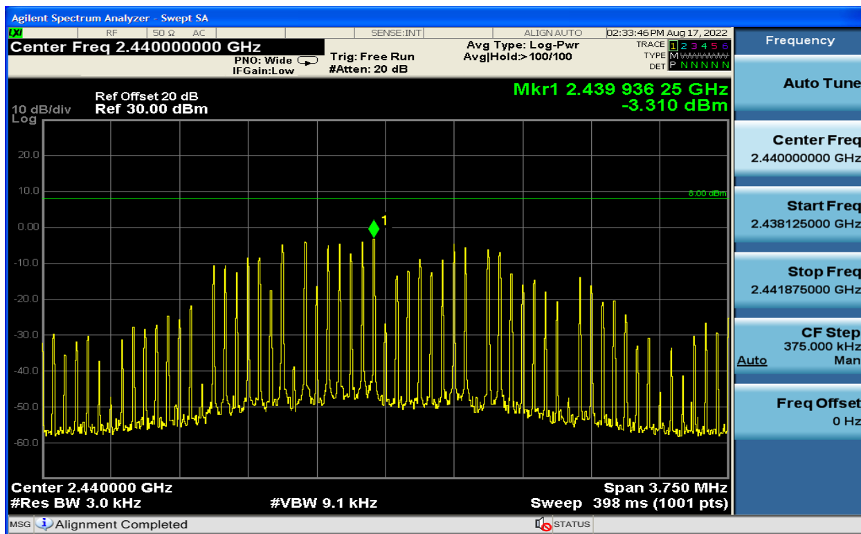
Plot 8-2: Power Spectral Density – 2440 MHz
