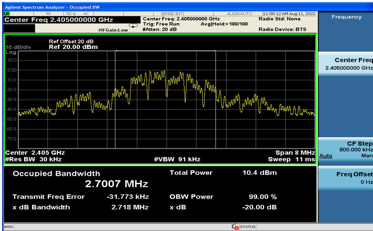
Plot 6-1: 99% Bandwidth, 2405 MHz
