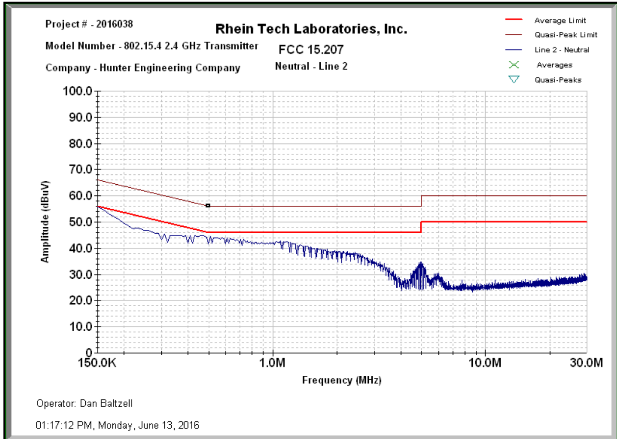
Plot 8-1: Conducted Emissions Test Data – Neutral - TX Mode
