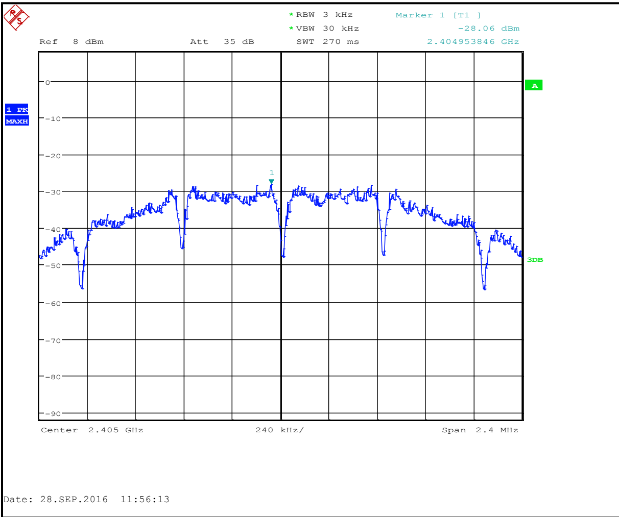
Plot 7-1: Power Spectral Density – 2405 MHz
