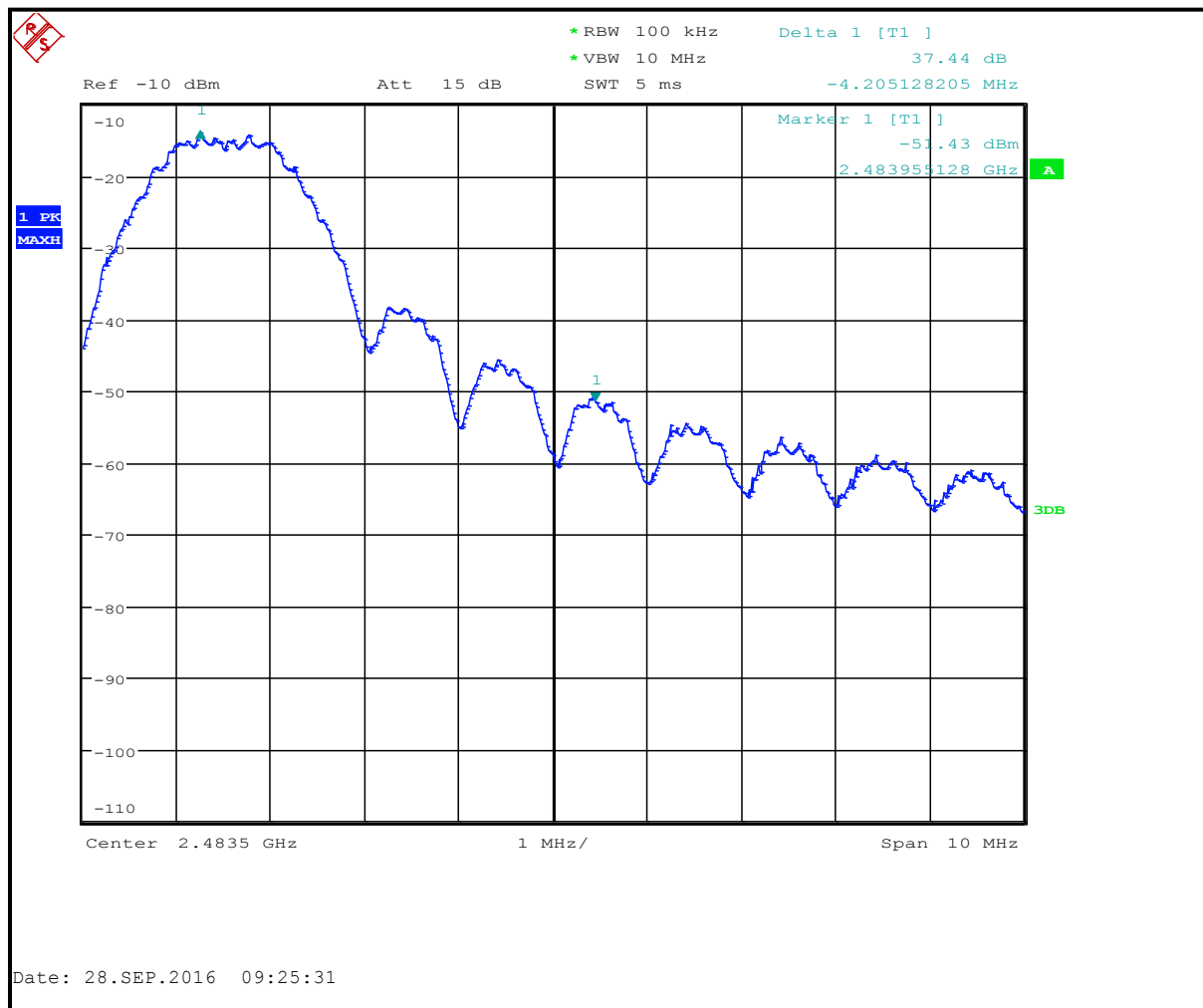
Plot 4-2: Upper Band Edge
