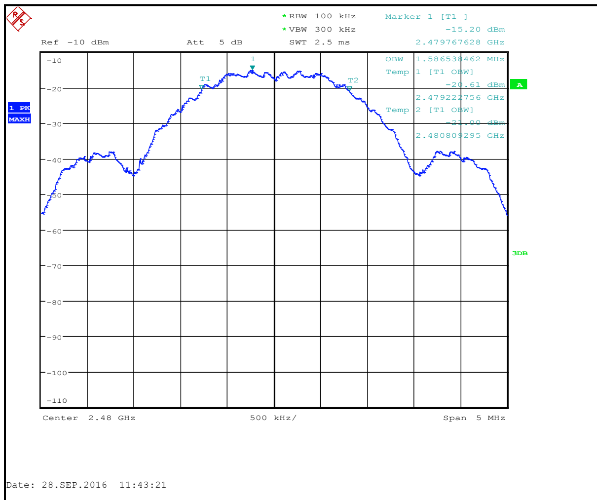
Plot 6-3: 6 dB Bandwidth – 2480 MHz
