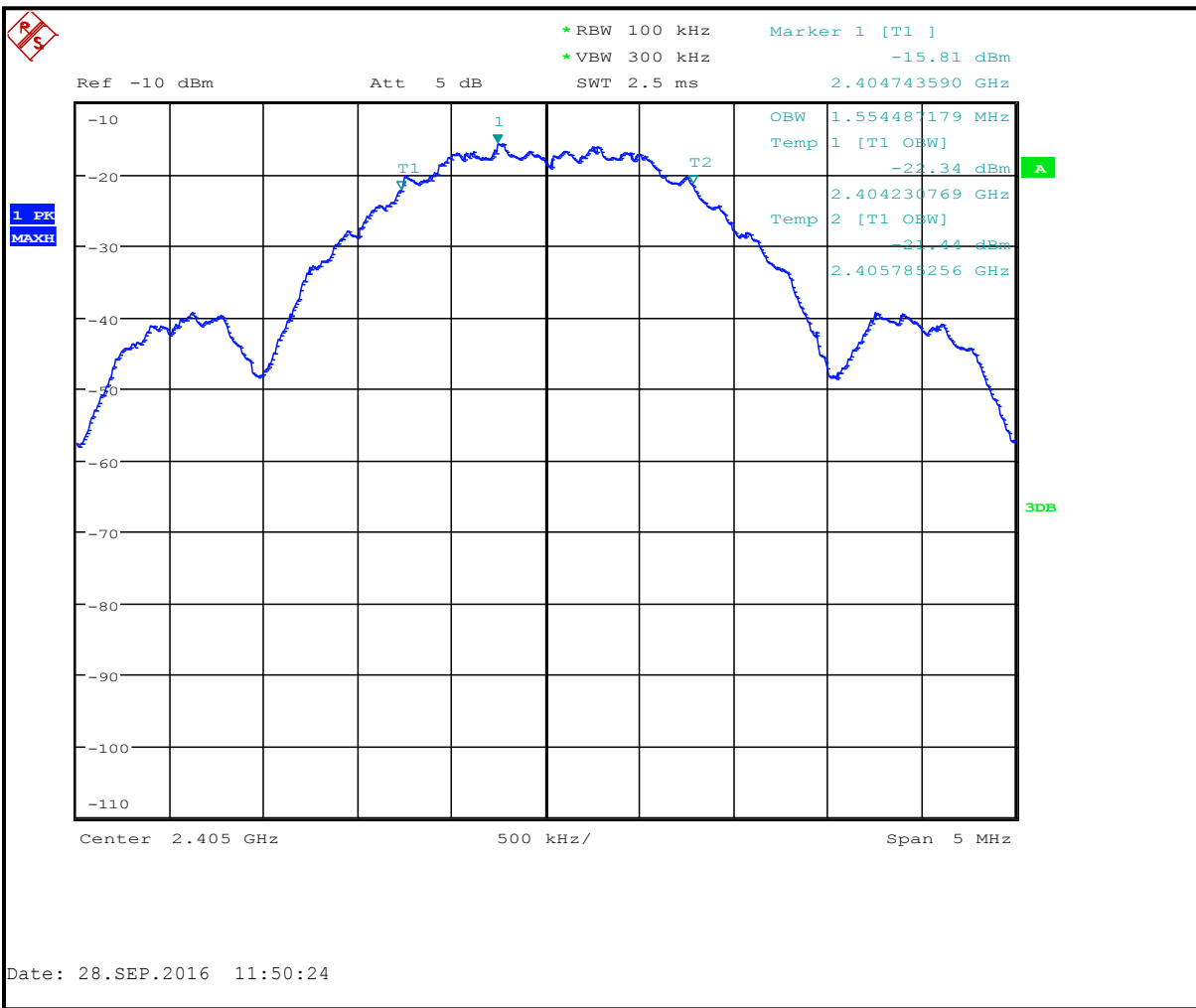
Plot 6-1: 6 dB Bandwidth – 2405 MHz
