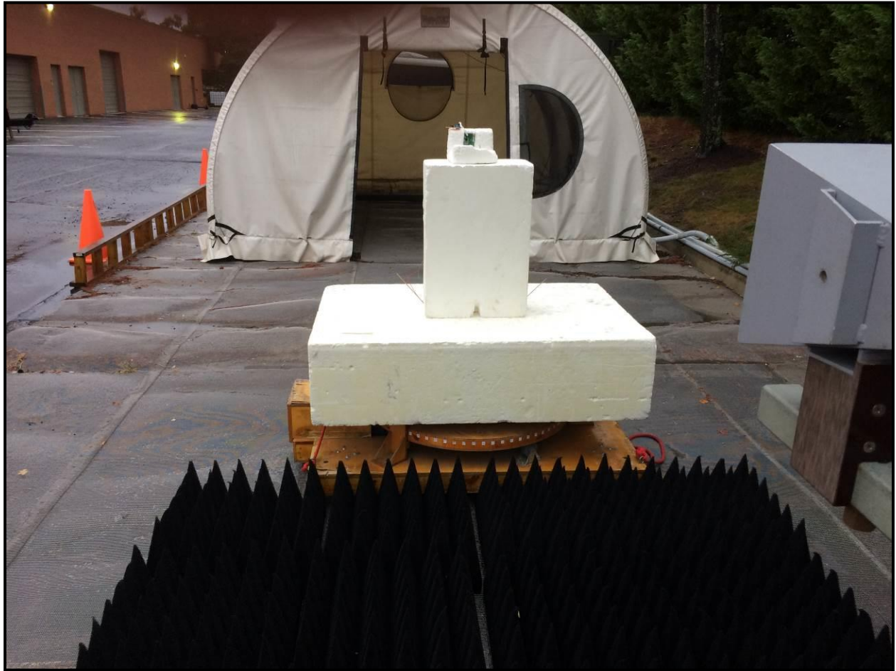
Photograph 4: Radiated Emissions Testing – Front View (> 1 GHz)
