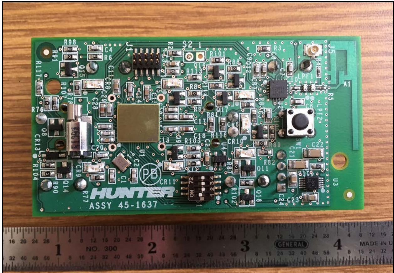
Photograph 5: Module with Shield – Front View
