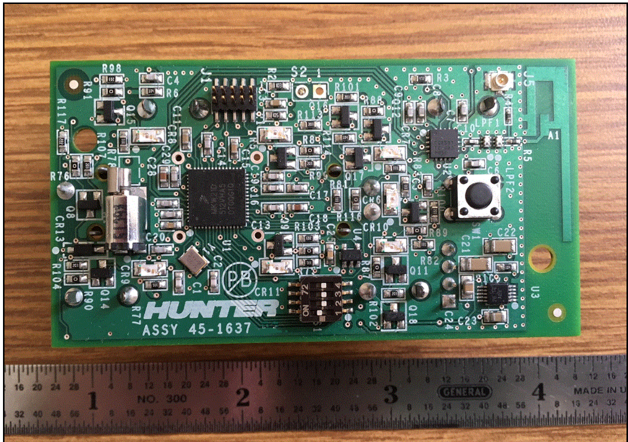
Photograph 6: Module without Shield - Front View
