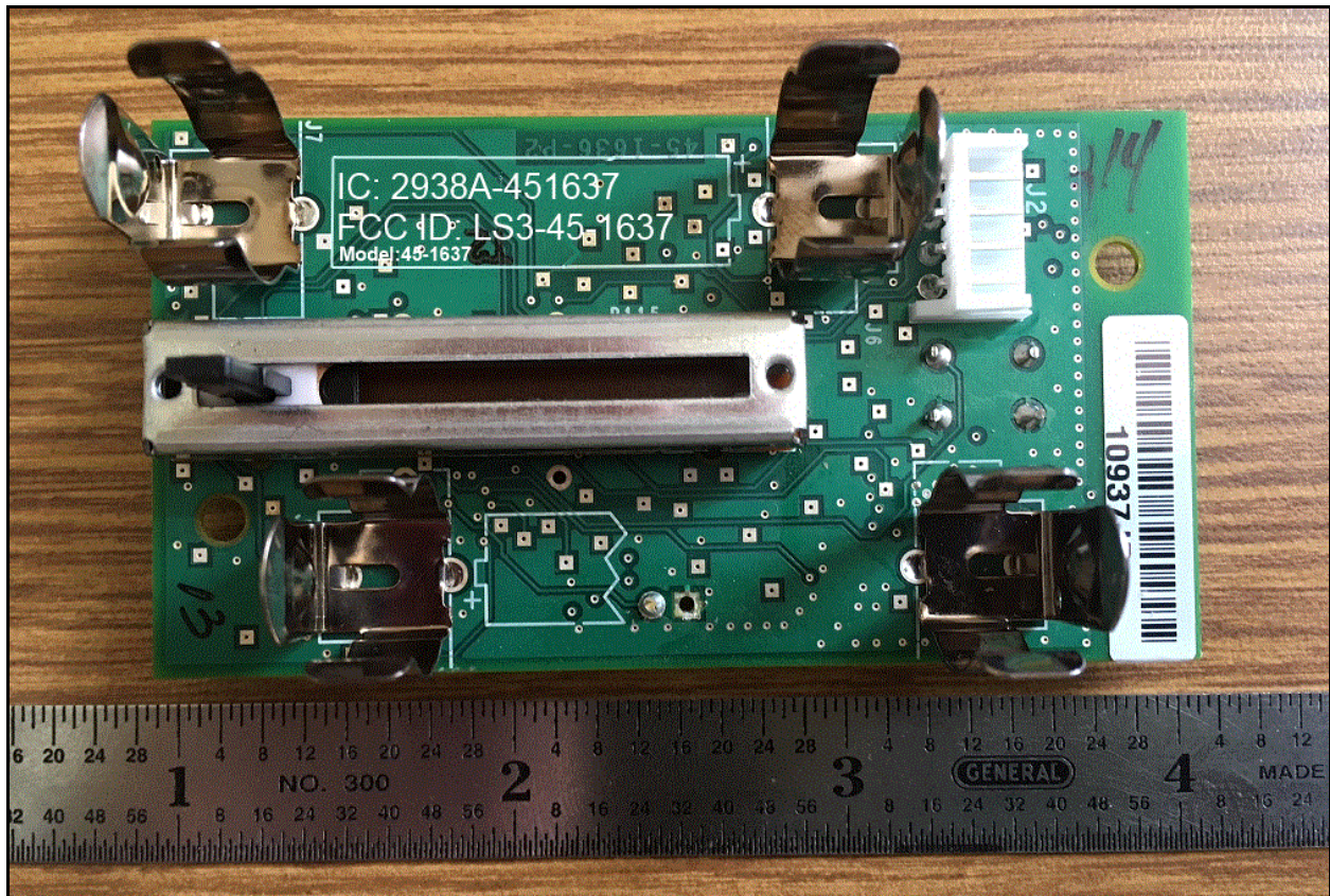
Photograph 7: Module – Back View
