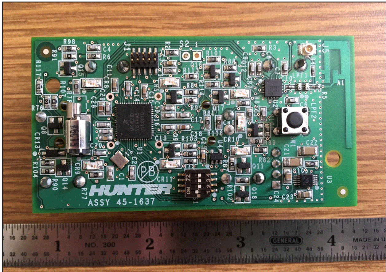
Photograph 9: Module without Shield - Front View
