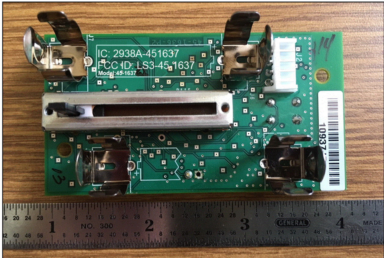
Photograph 10: Module – Back View
