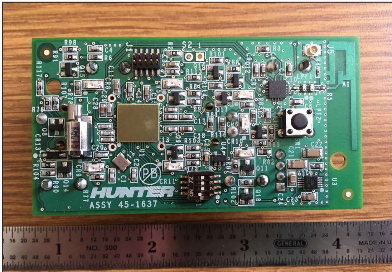
Photograph 8: Module with Shield – Front View
