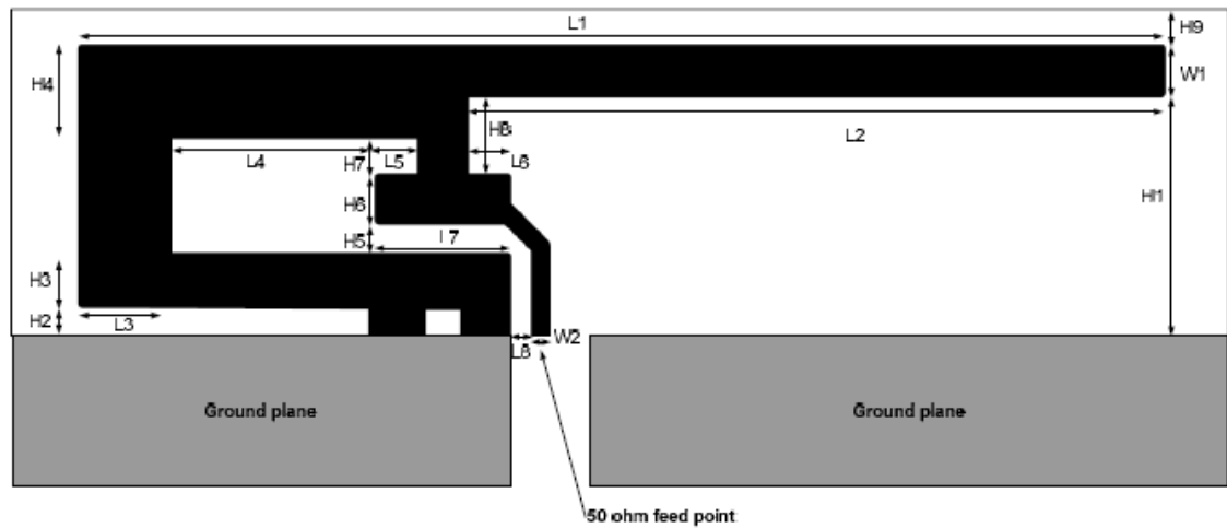
Figure 1. IFA Dimensions
