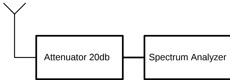
Figure- 1 Bandwidth test setup
