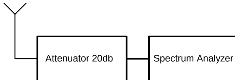
Figure- 2 Field strength of fundamental test setup
