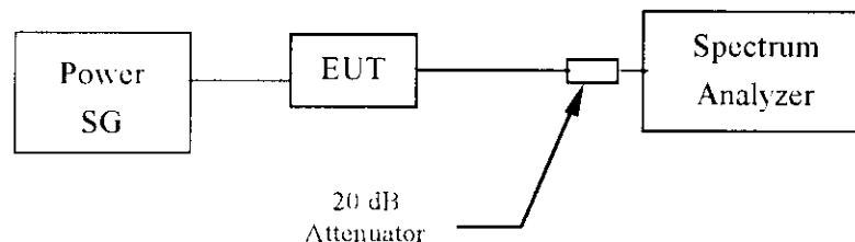
Figure 1 : Output power measurement configuration
