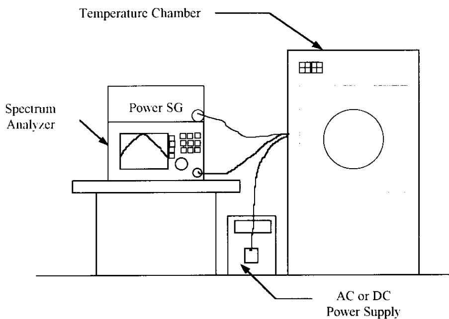
Figure 5 : Frequency stability measurement configuration
