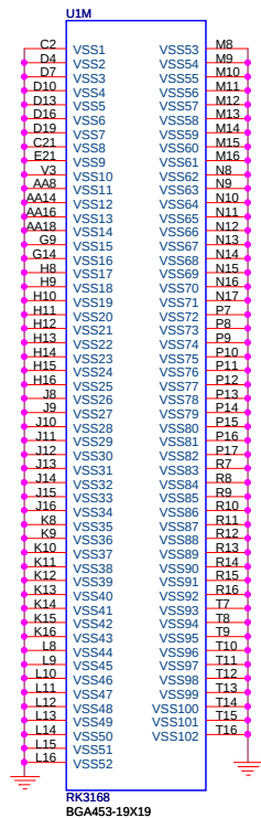
RK3168_M
