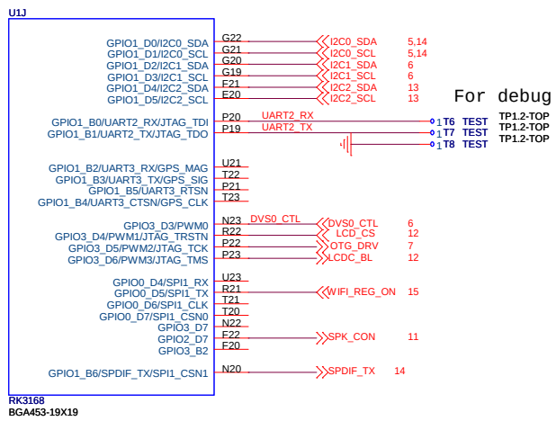
RK3168_J
