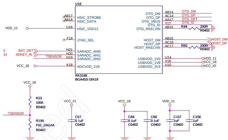
RK3168_E
