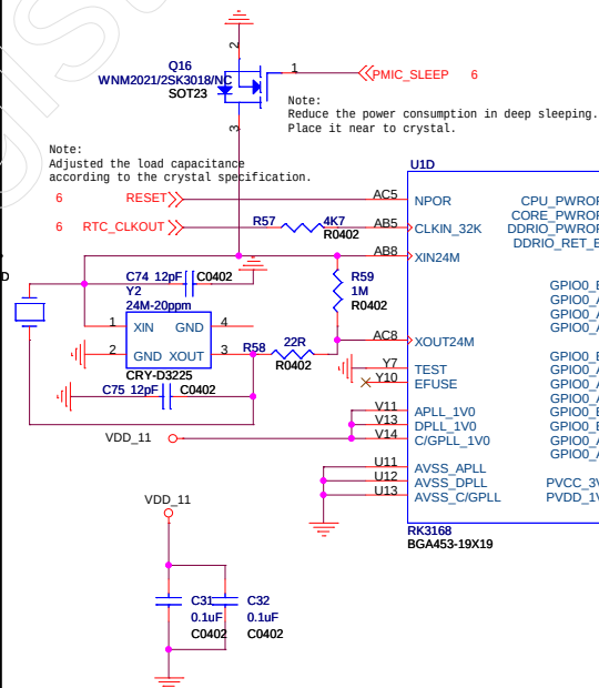
RK3168_D
