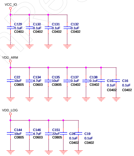
RK3188 CORE POWER FILTER
