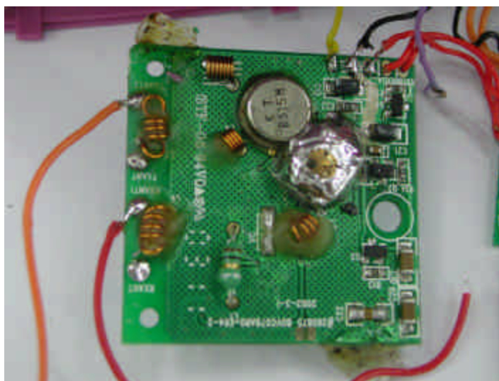
Internal Photo – 5
