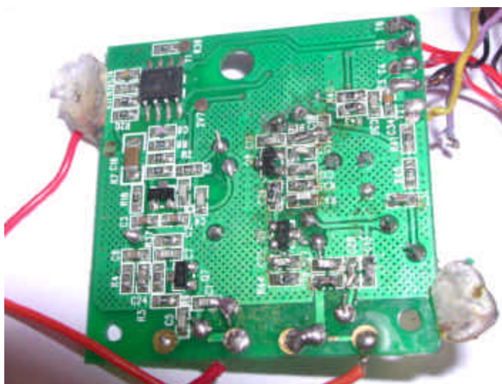
Internal Photo – 6
