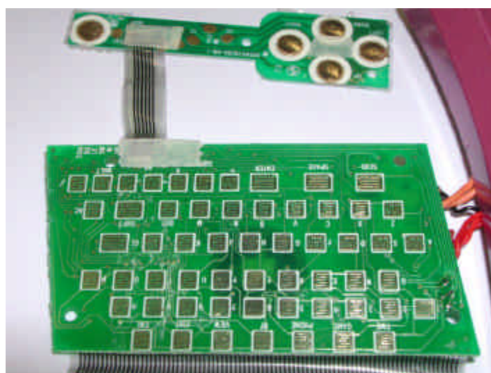
Internal Photo – 4
