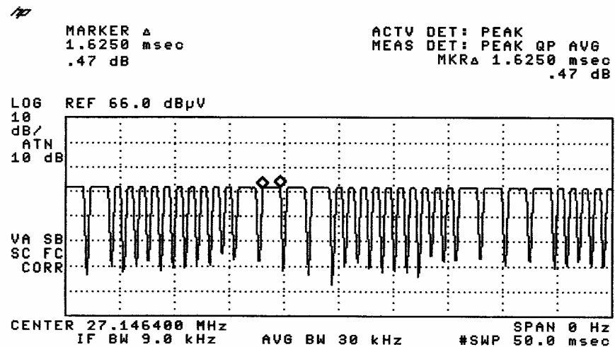
Figure C [Long Pulse]
