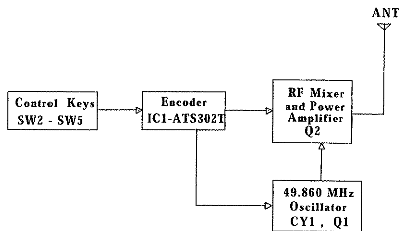
TX 49.860MHz FUNCTION BLOCK DIAGRAM
