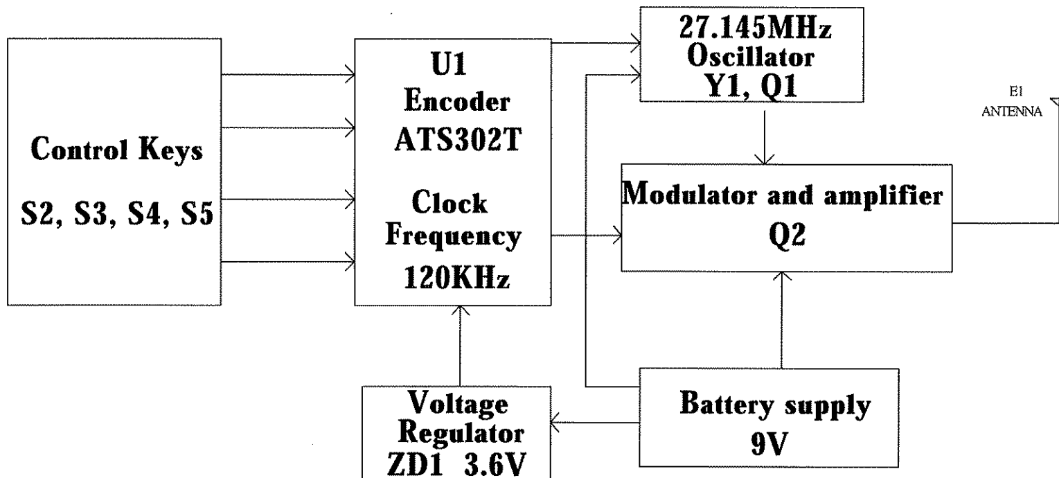
Block diagram Product number :338376 Transmitter 27.145MHz
