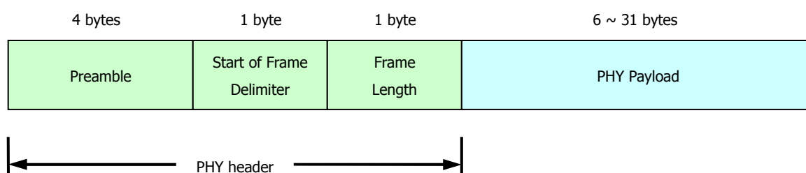
Figure 4. PHY Layer Frame Format
