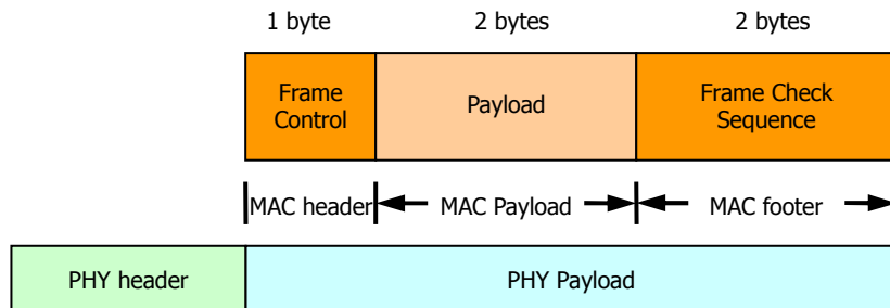
Figure 7. Acknowledgement Frame Format
