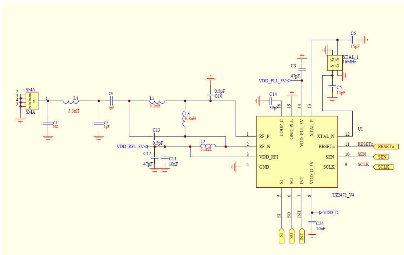
Figure 17-1. UM2471 Reference Circuit (#1)
