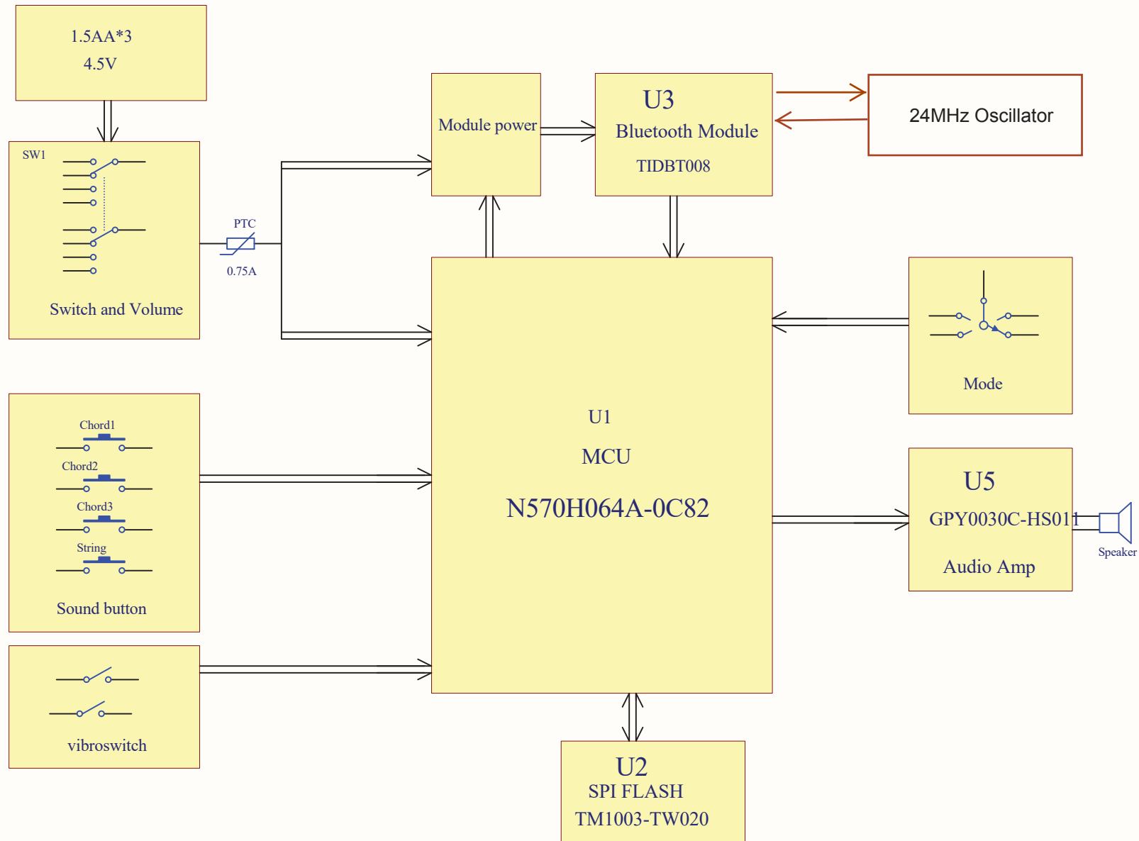
654794 Block diagram
