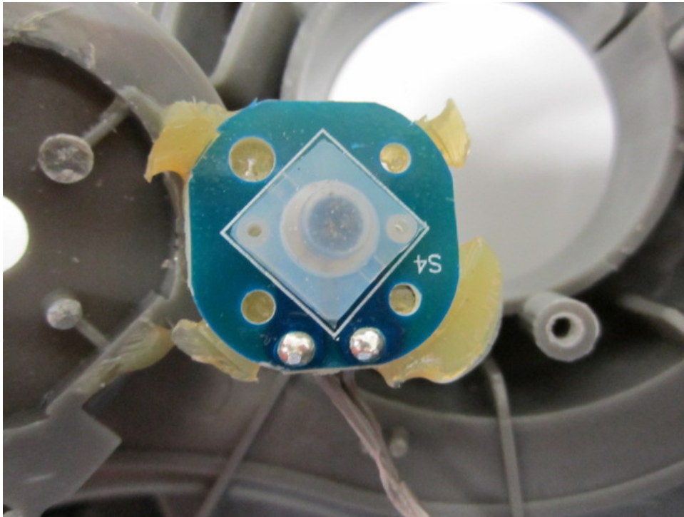
1.1.17 Internal view 14
