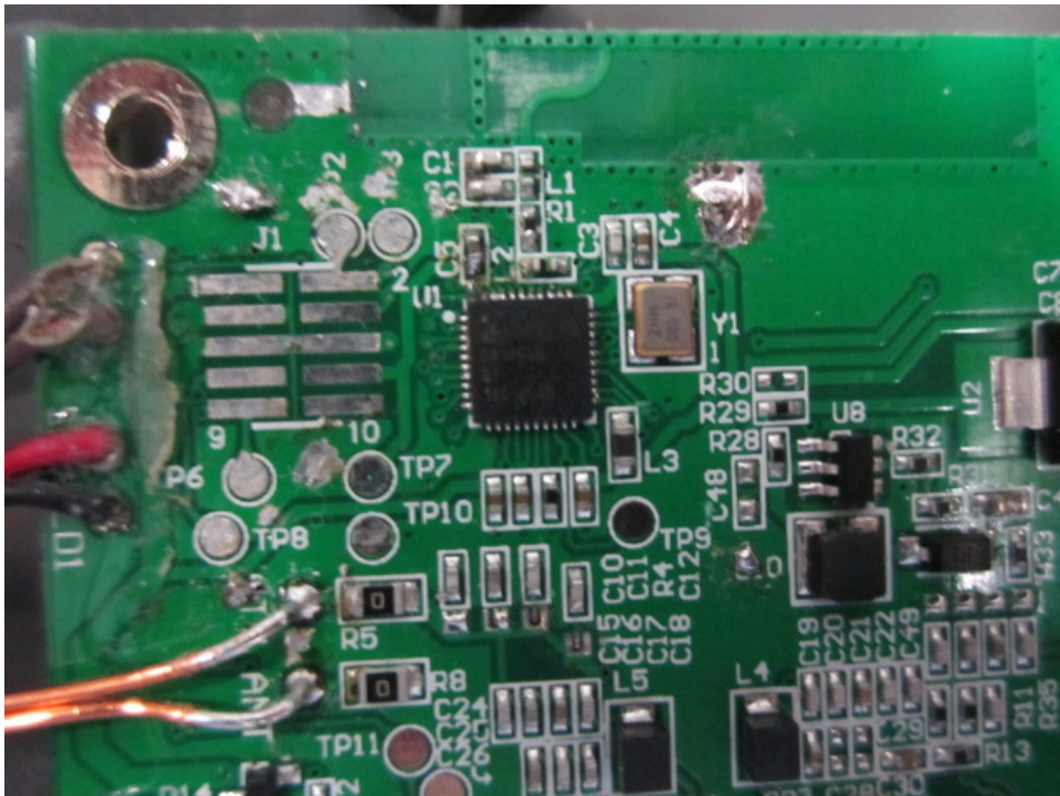
1.1.7 Internal view 4
