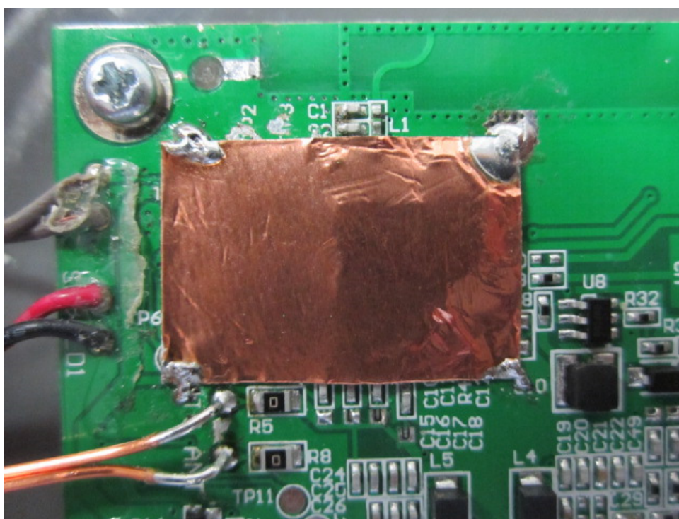
Internal View
