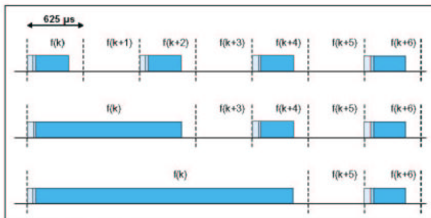
Figure 2.2: Multi-slot packets
