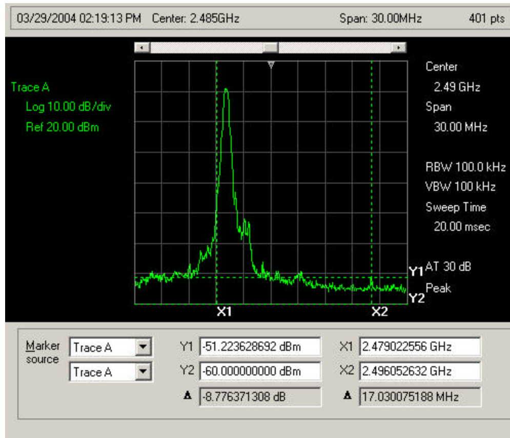
Plot 15: Band-edge compliance, Upper Band-edge (Hopping Disabled)
