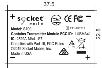
DETAIL A SCALE 1:1 REF. ONLY
