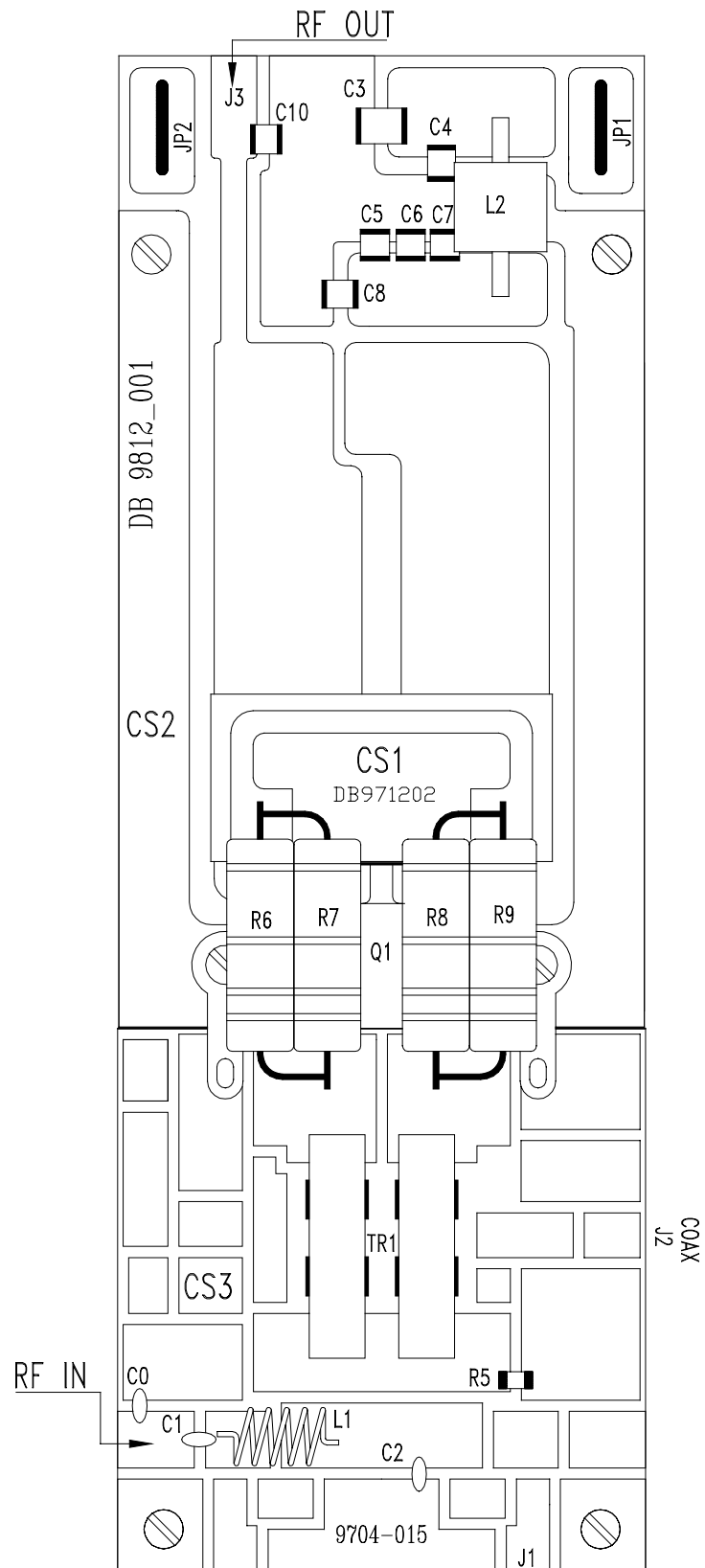
Fig. 9.2 - AMP300 AMPLIFIER COMPONENT LAYOUT (DB 9812_001)
