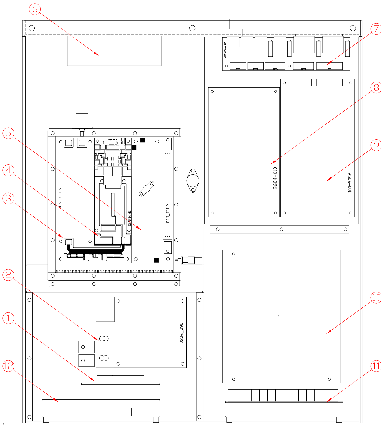
Fig. 1.3 - TOP VIEW
