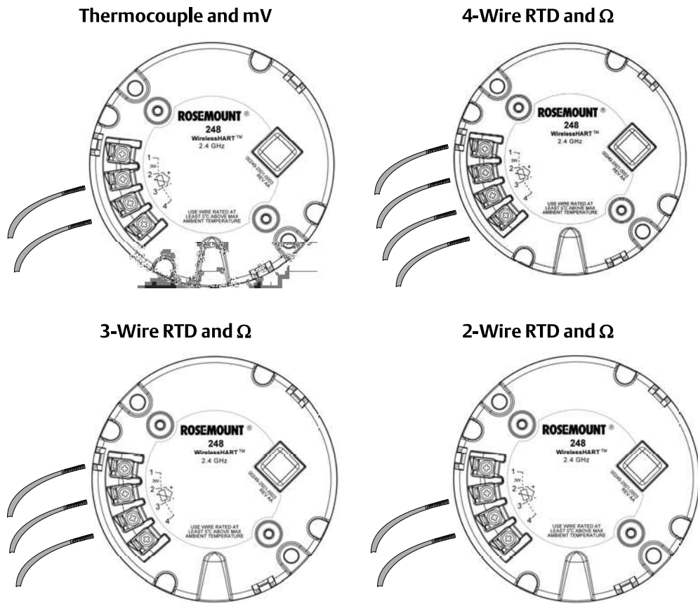
Figure 2-1. Sensor Wiring
