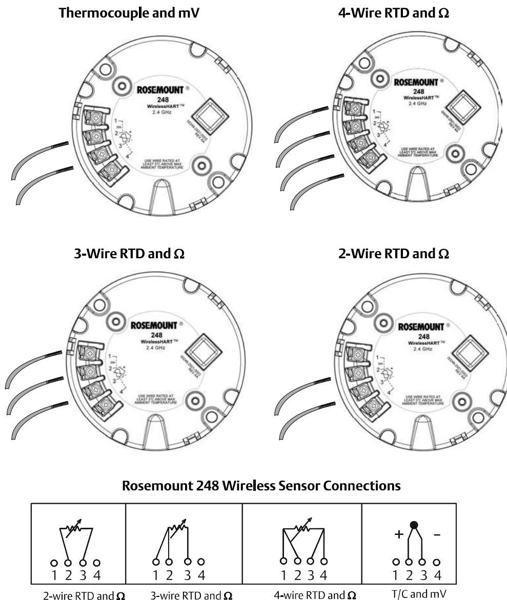
Figure 4-3. Sensor Wiring
