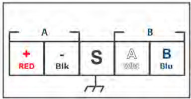
Figure 3-2: Wiring Guide
