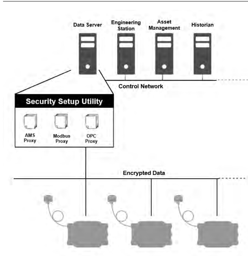
Figure 4-1: Typical Host System Architecture Using Security Setup
