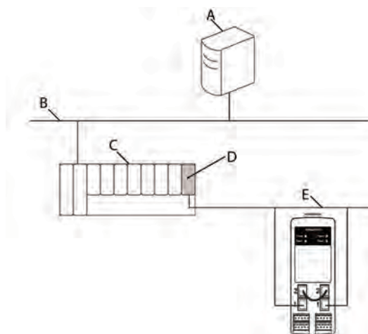
Figure B-6: Simplex RS-485 Architecture
