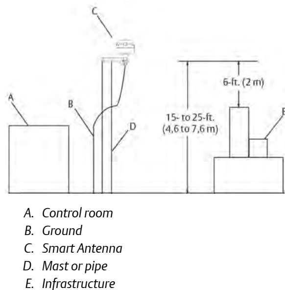
Figure 3-3: Mounting Location
