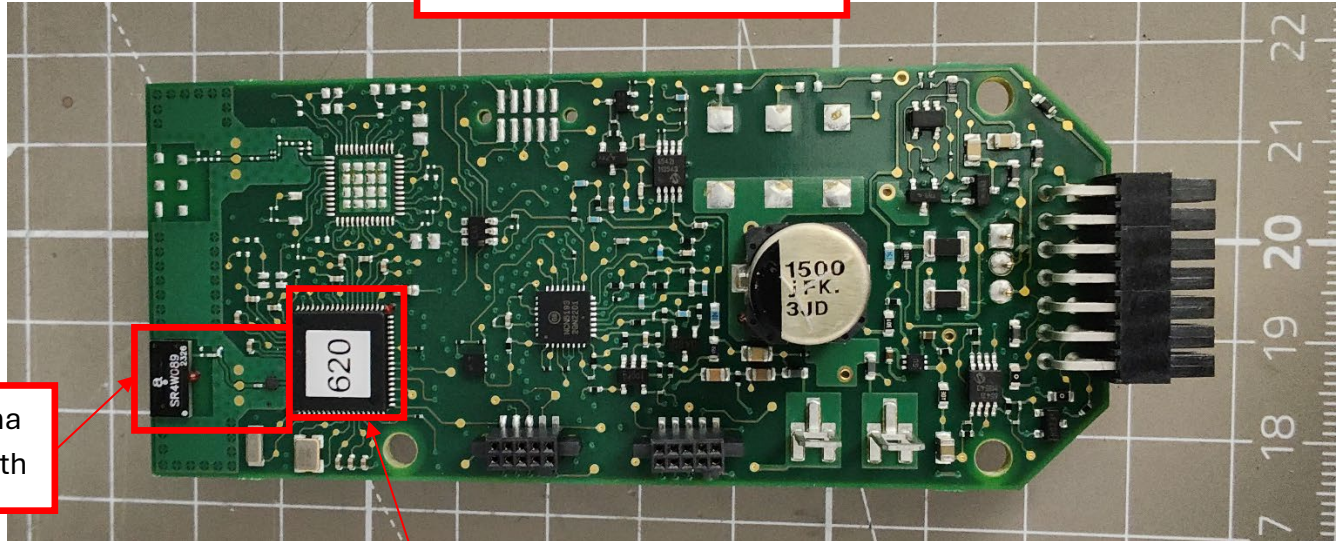
CM Board - Top View
