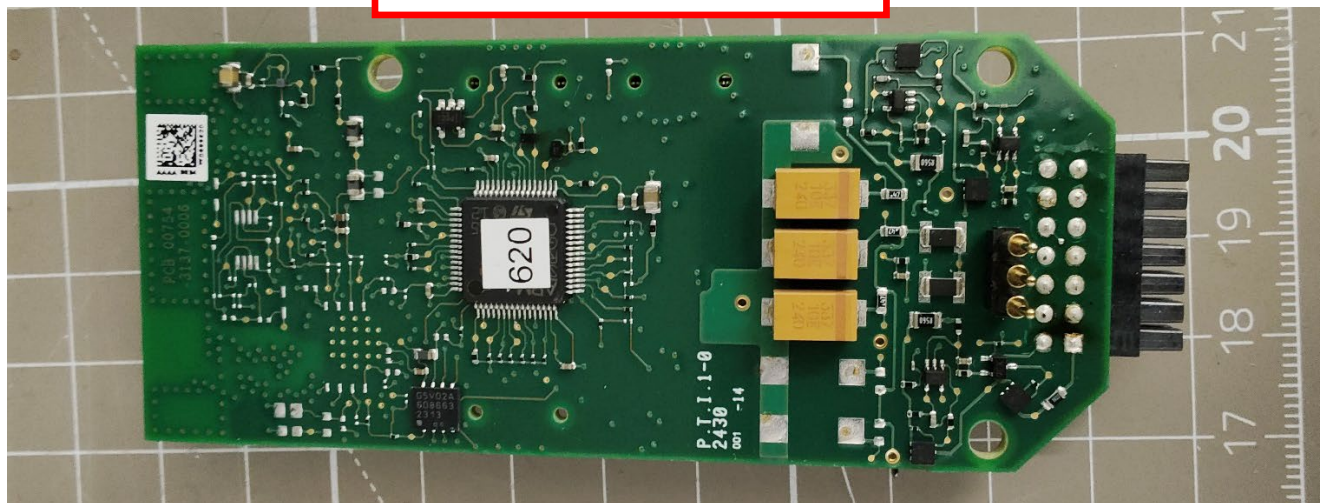
CM Board - Bottom View
