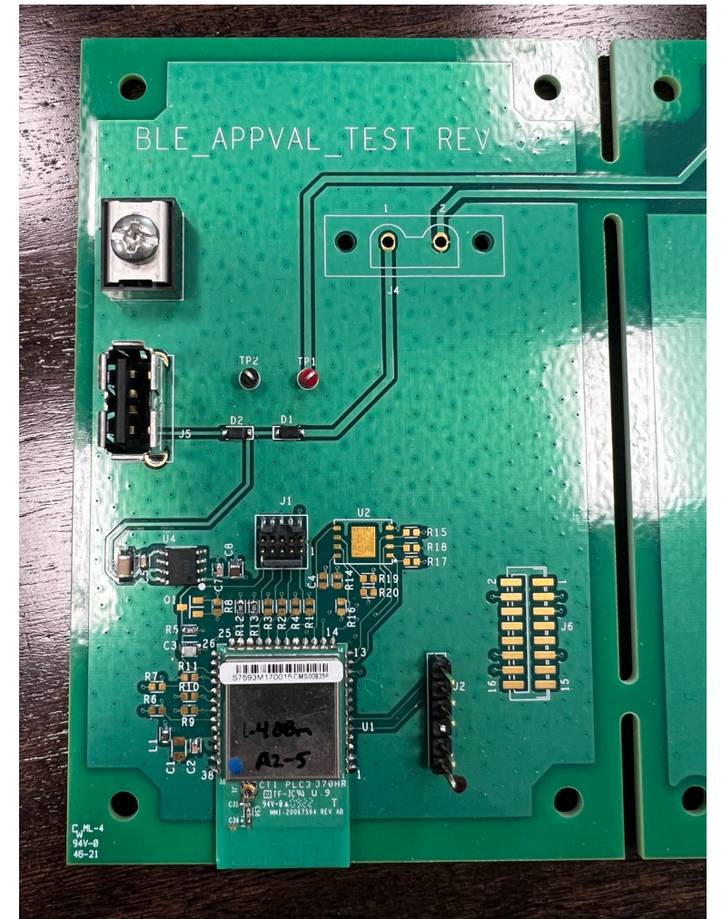
Module on test board
