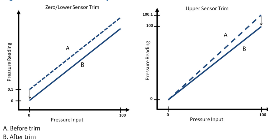
Figure 4-1. Sensor Trim Example
