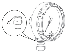
Figure 2-3. Low Side Pressure Port
