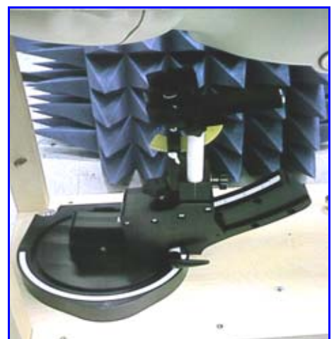
Figure 9. Device Holder
