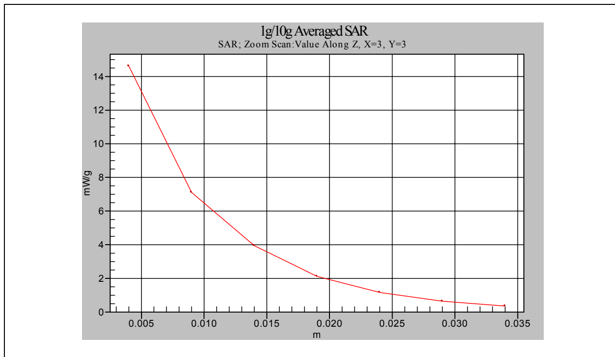
Body-Tissue-Simulating-Liquid 2450MHz
