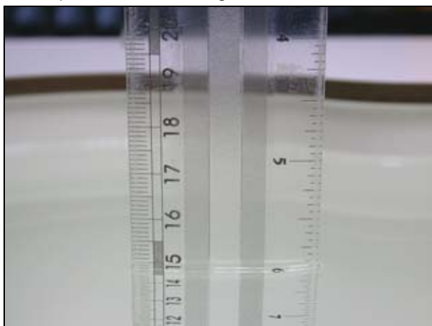
Figure 11. Head-Tissue-Simulating-Liquid 2450MHz
