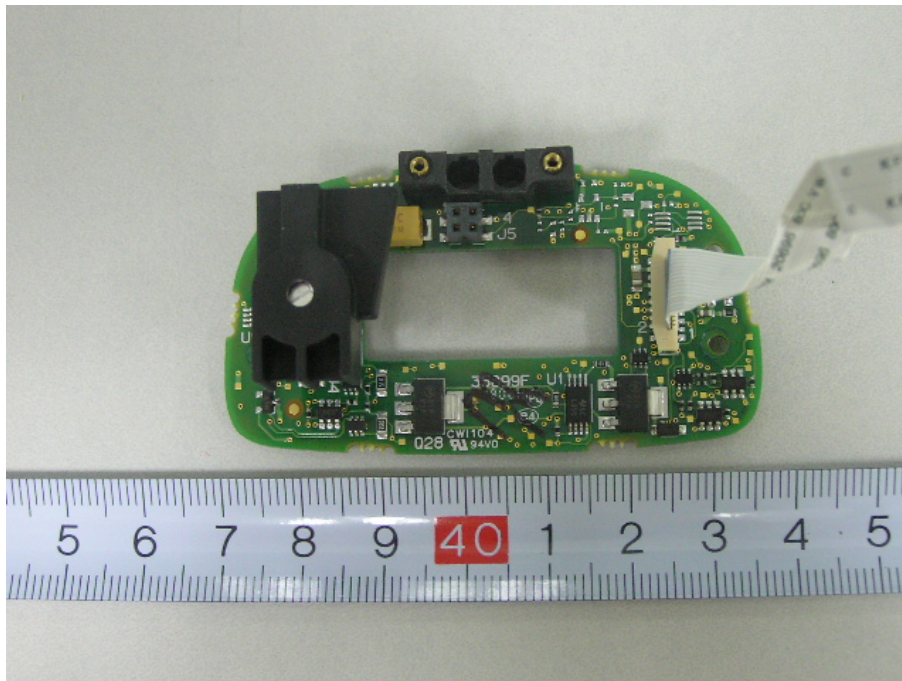
35899F –PCB Top View
