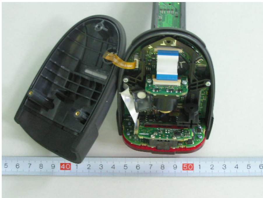
EUT –Inside View (4)
