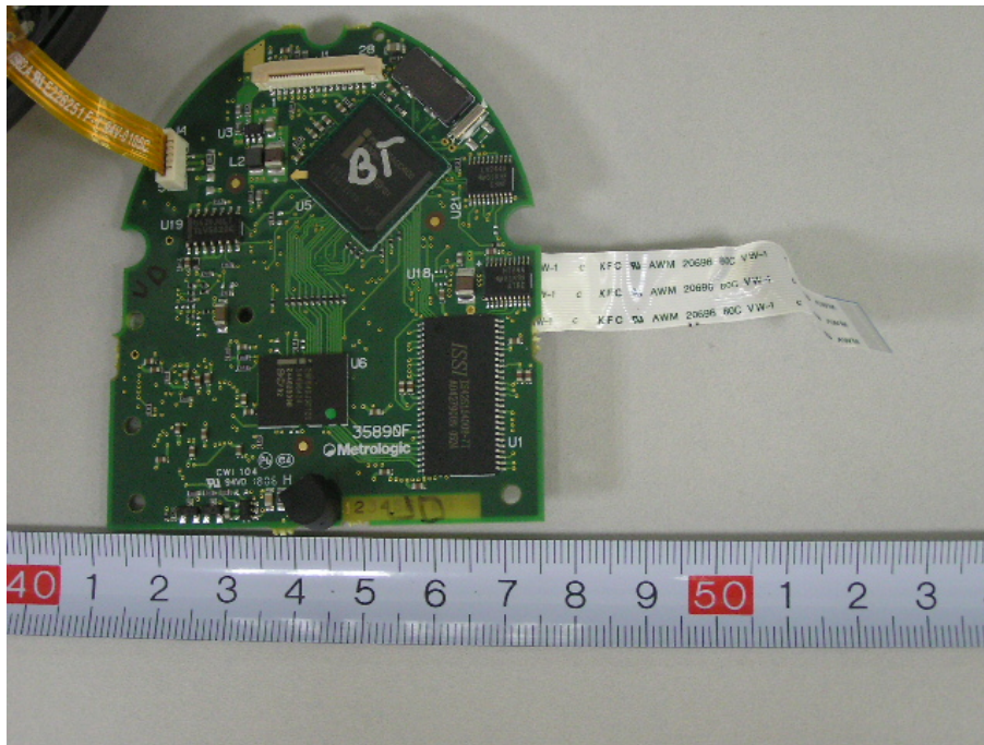
35890 –PCB Top View
