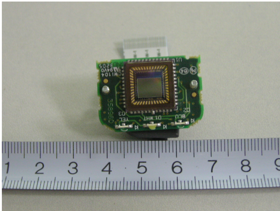
35896D –PCB Top View
