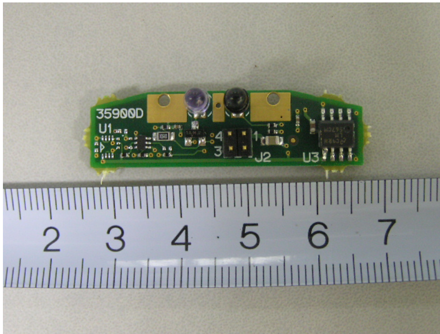
35900D –PCB Top View
