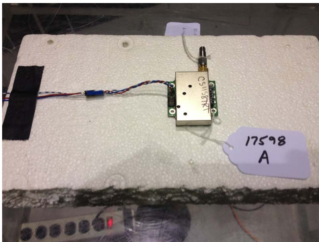
Radiated Emissions, Close-up
