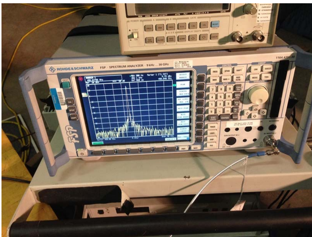
Frequency Measurement Setup
