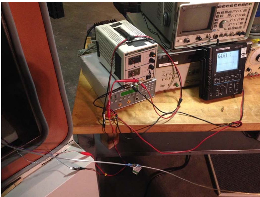
EUT Temperature/Voltage Equipment Setup
