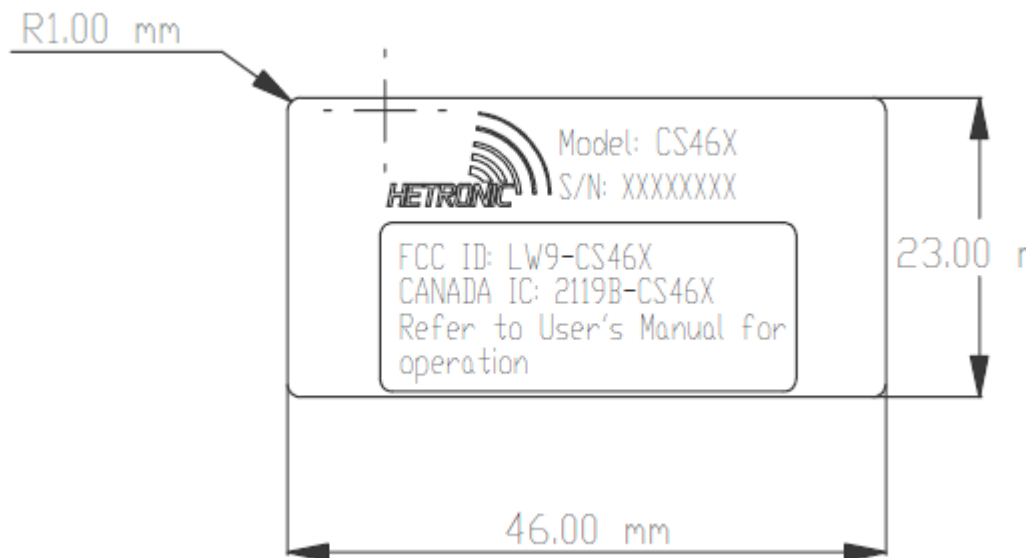
Figure 2, Module Label
