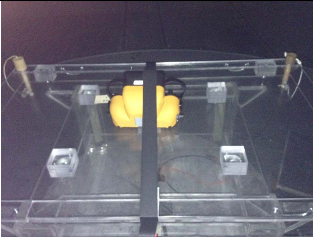
Radiated Spurious, Transmit Mode. Rear, Maximum Emission Orientation
