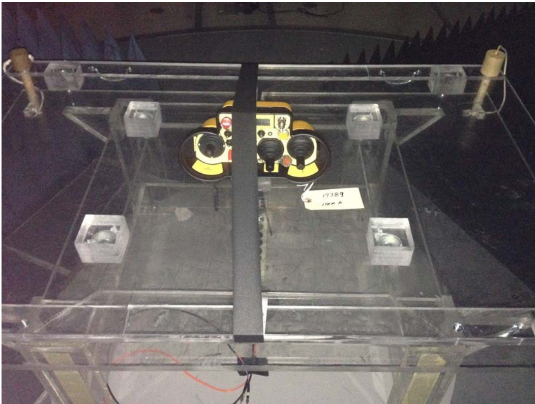
Radiated Spurious, Transmit Mode, Front, Maximum Emission Orientation
