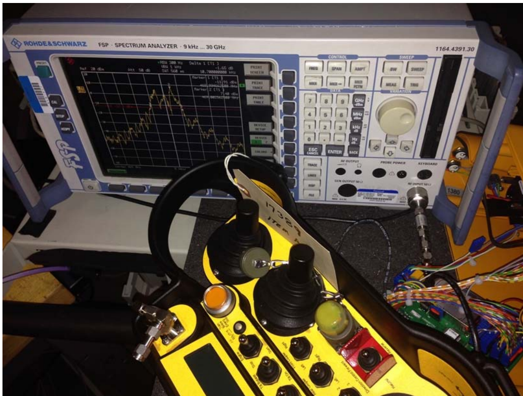
Conducted Port Measurements: Power, Spurious, Bandwidth
