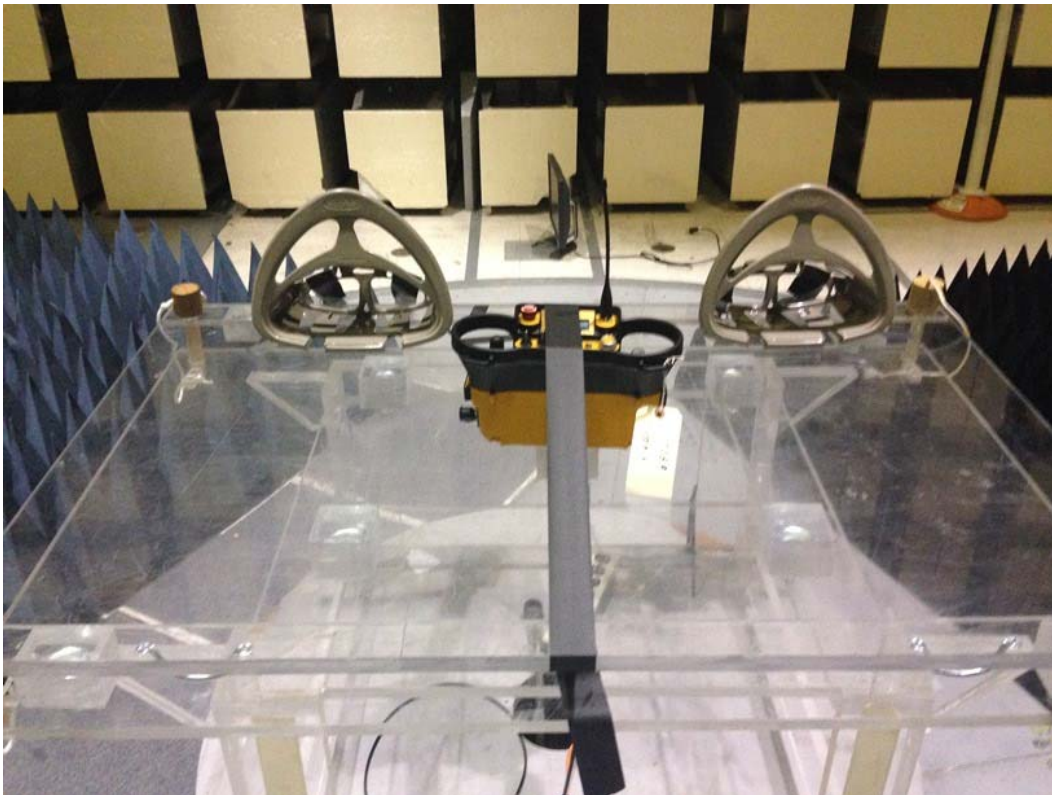
Radiated Spurious, Receive Mode, Front
