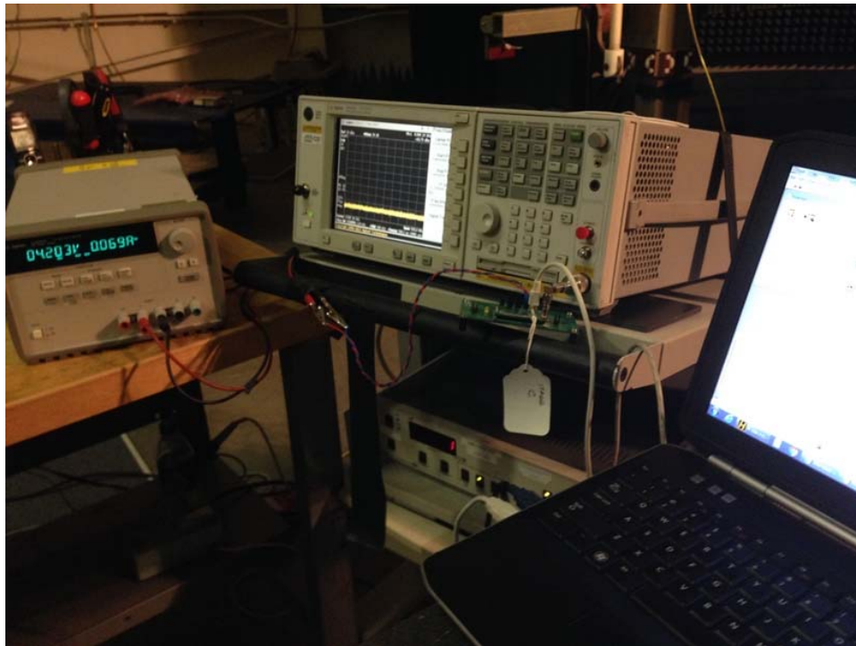
Conducted Antenna Port Spurious
