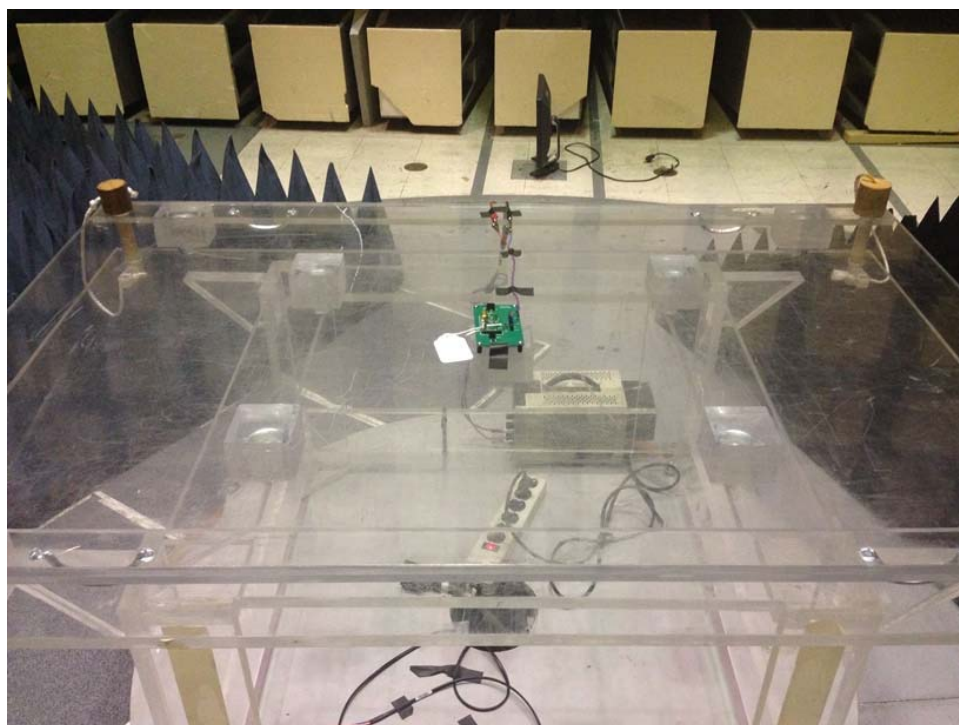
Radiated Emissions, Front
