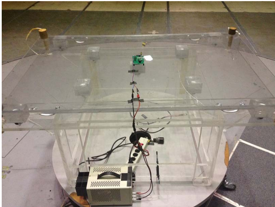
Radiated Emissions, Back
