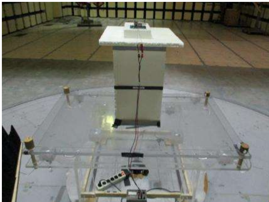
Radiated Emissions, Above 1 GHz, Back
