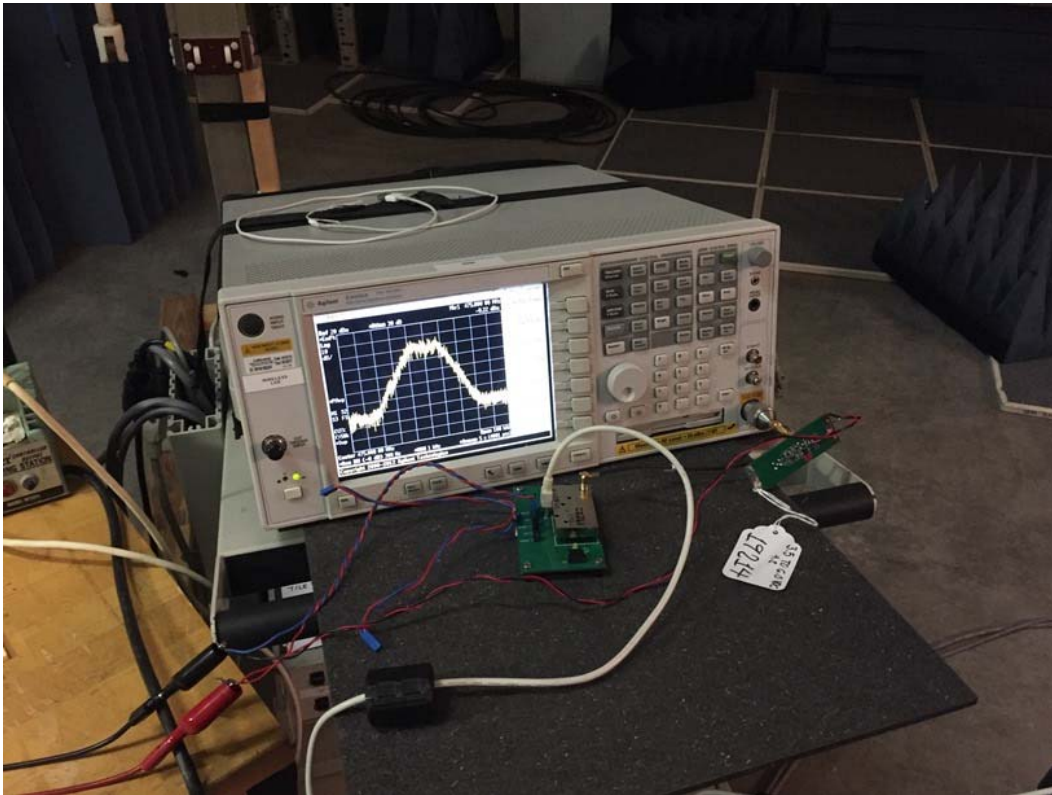
Conducted Measurements: Power, Masks, Spurious, Bandwidth
