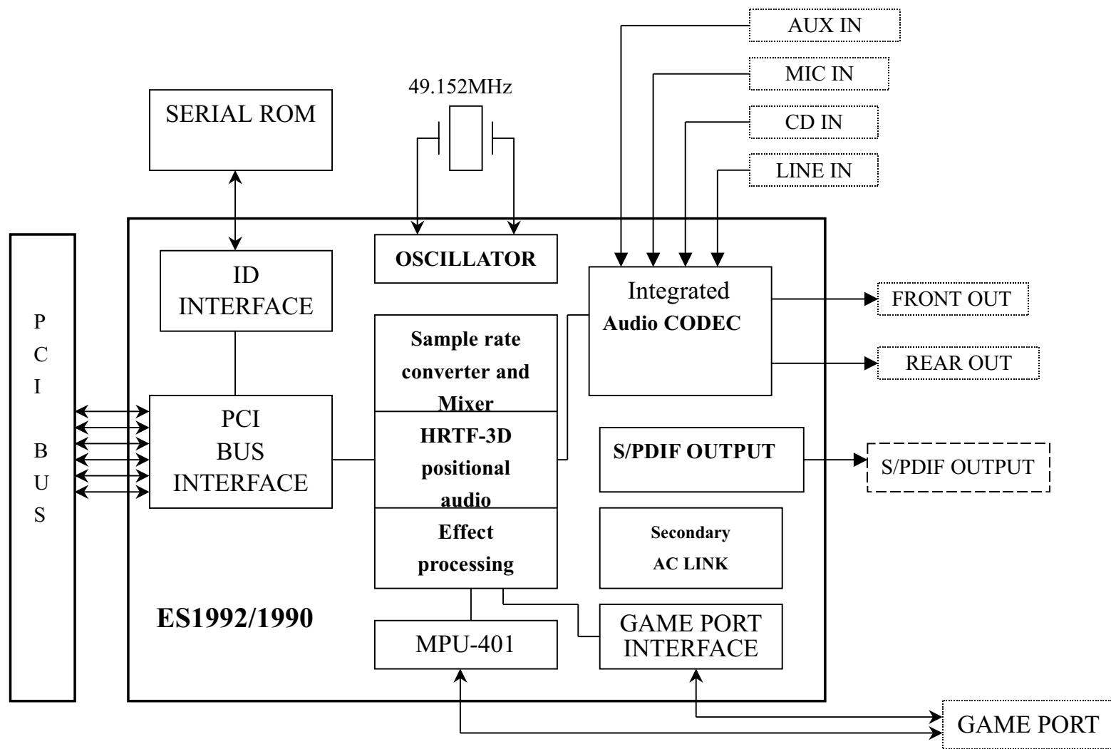
U70 BLOCK DIAGRAM
